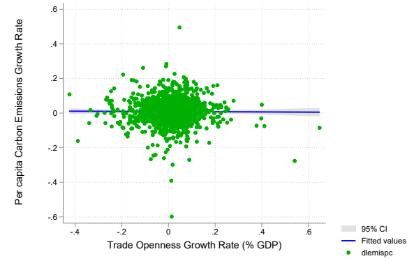
(e) Correlation dlemispc-dltrade
