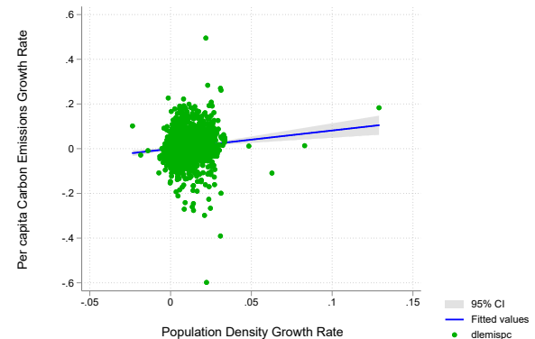
(g) Correlation dlemispc-dldensity
