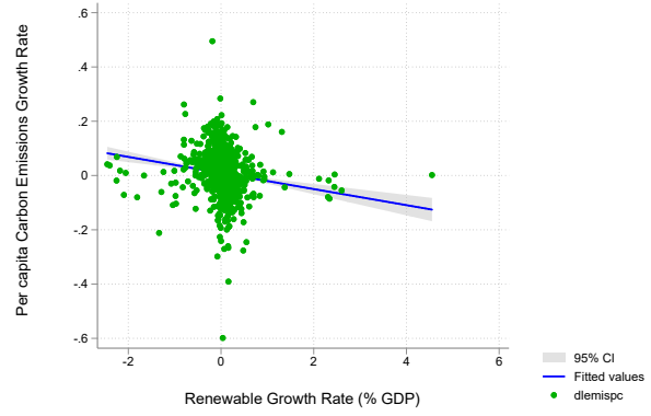
(b) Correlation dlemispc-dlrenew
