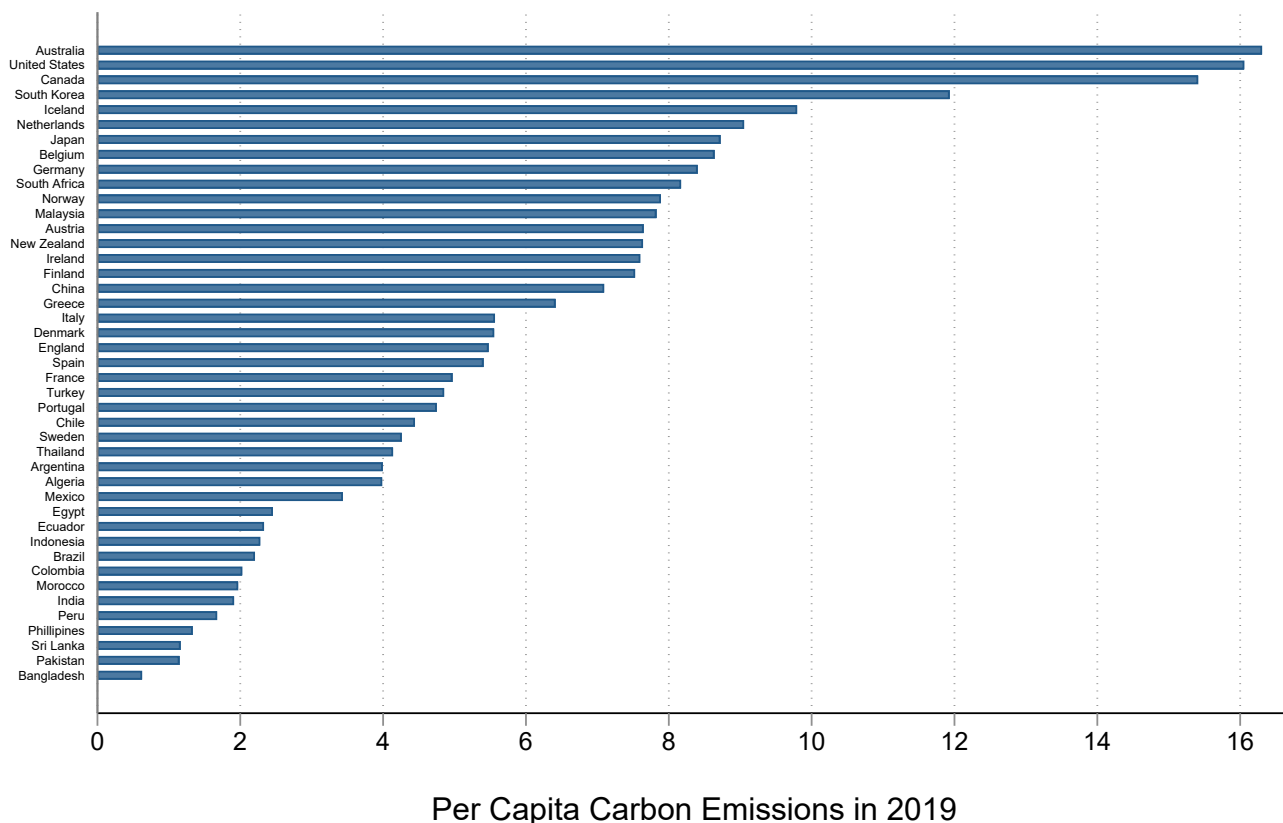
Figure 1: Per Capita Carbon Emissions in year 2019.
