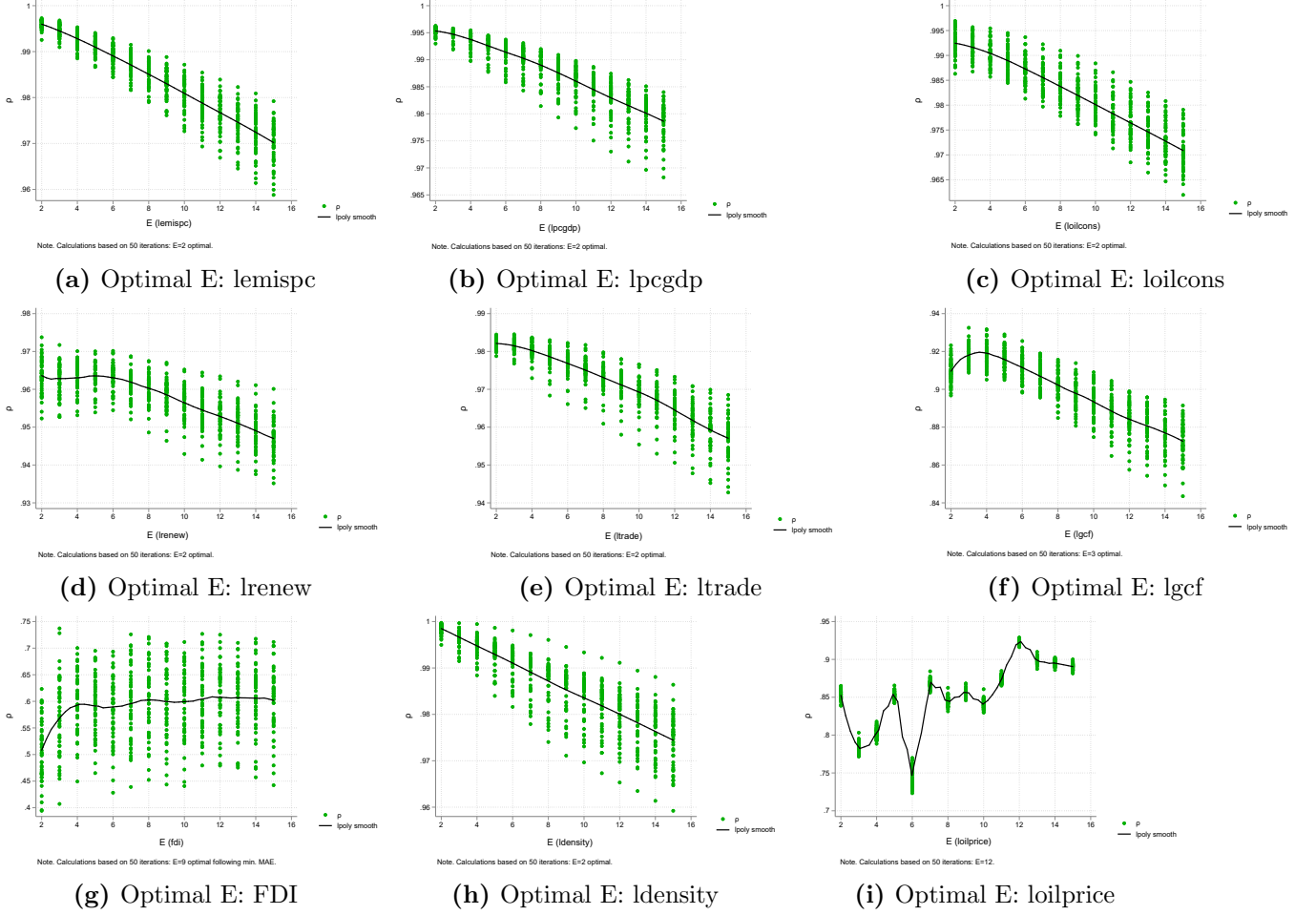
Figure 3: Selection of Optimal E.
