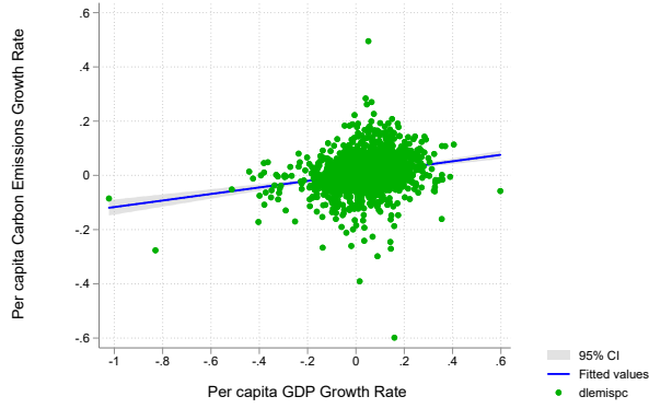
(a) Correlation dlemispc-dlpcgdp 2
