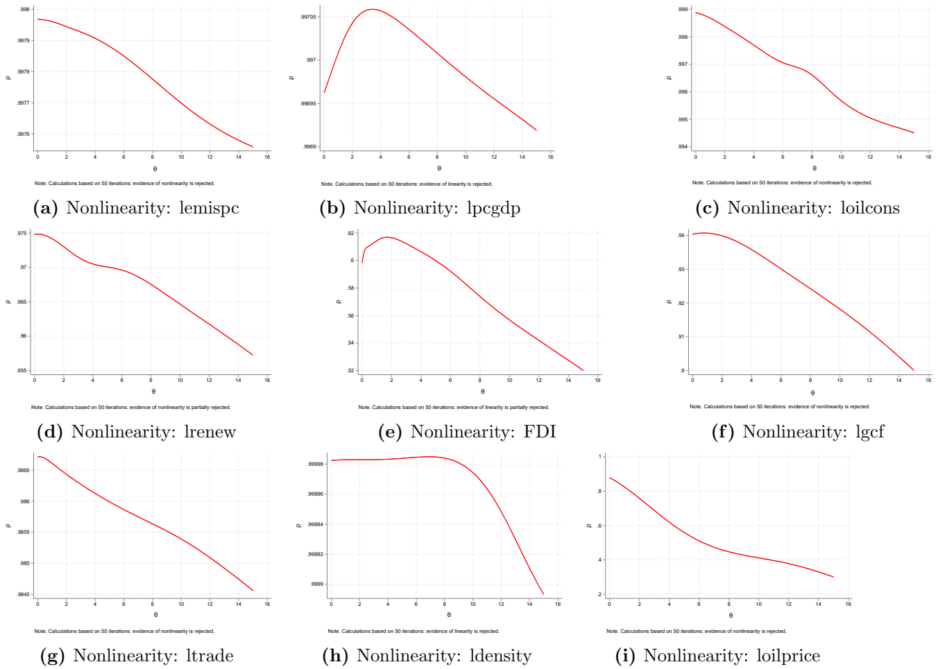
Figure 4: Testing for nonlinearity of variables.
