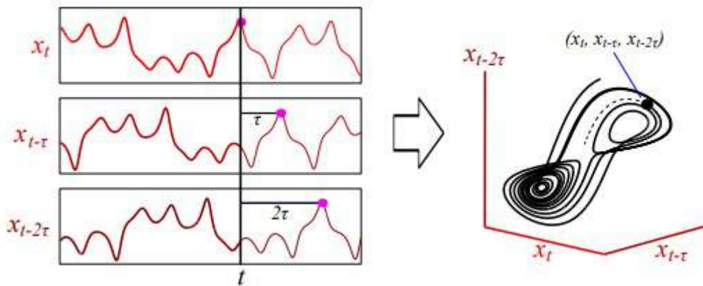
Figure 7: An example of manifold reconstruction.
