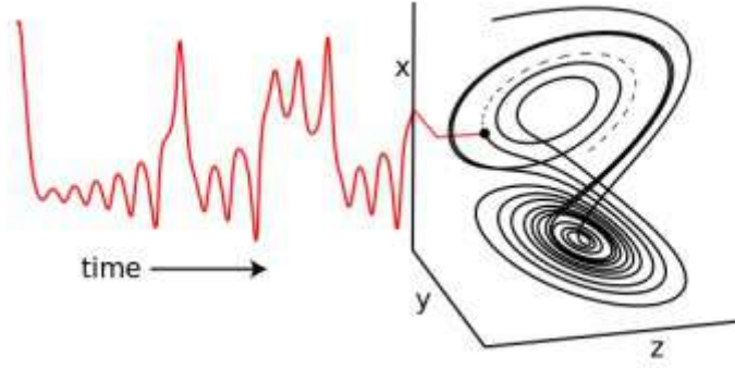
Figure 6: Time Series Projection from the Lorenz Attractor.
