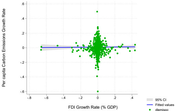
(c) Correlation dlemispc-dfdi
