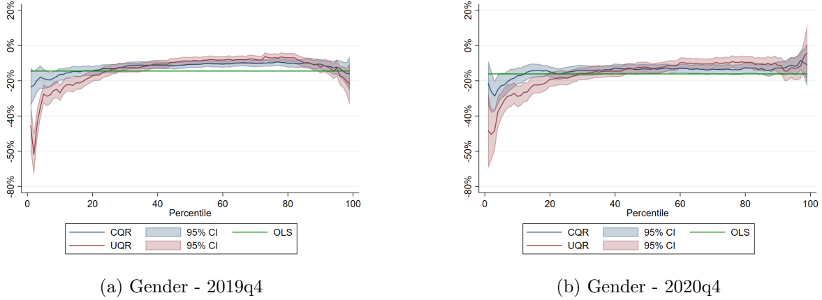
Figure 5: Marginal effects: OLS, CQR and UQR, Gender Gap
