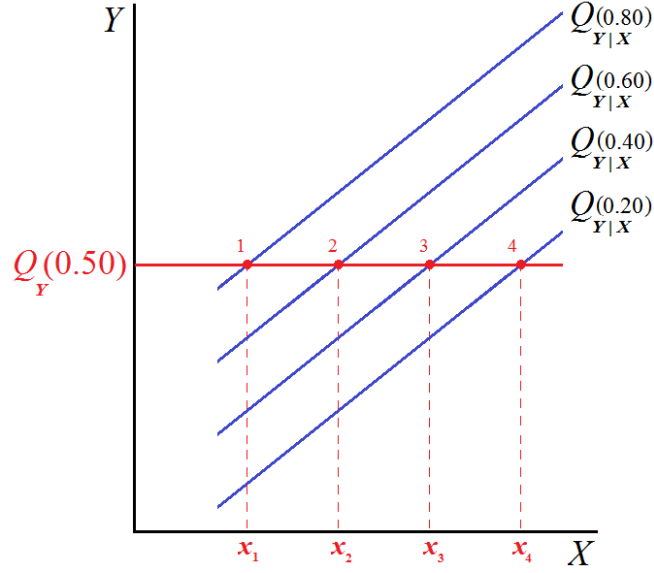
Figure 2: Linear location-shift model
