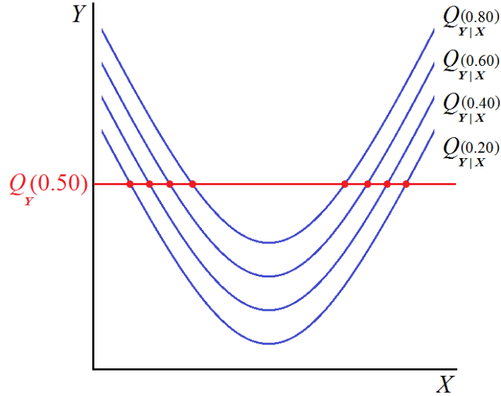
Figure 3: Nonlinear quadratic location-shift model
