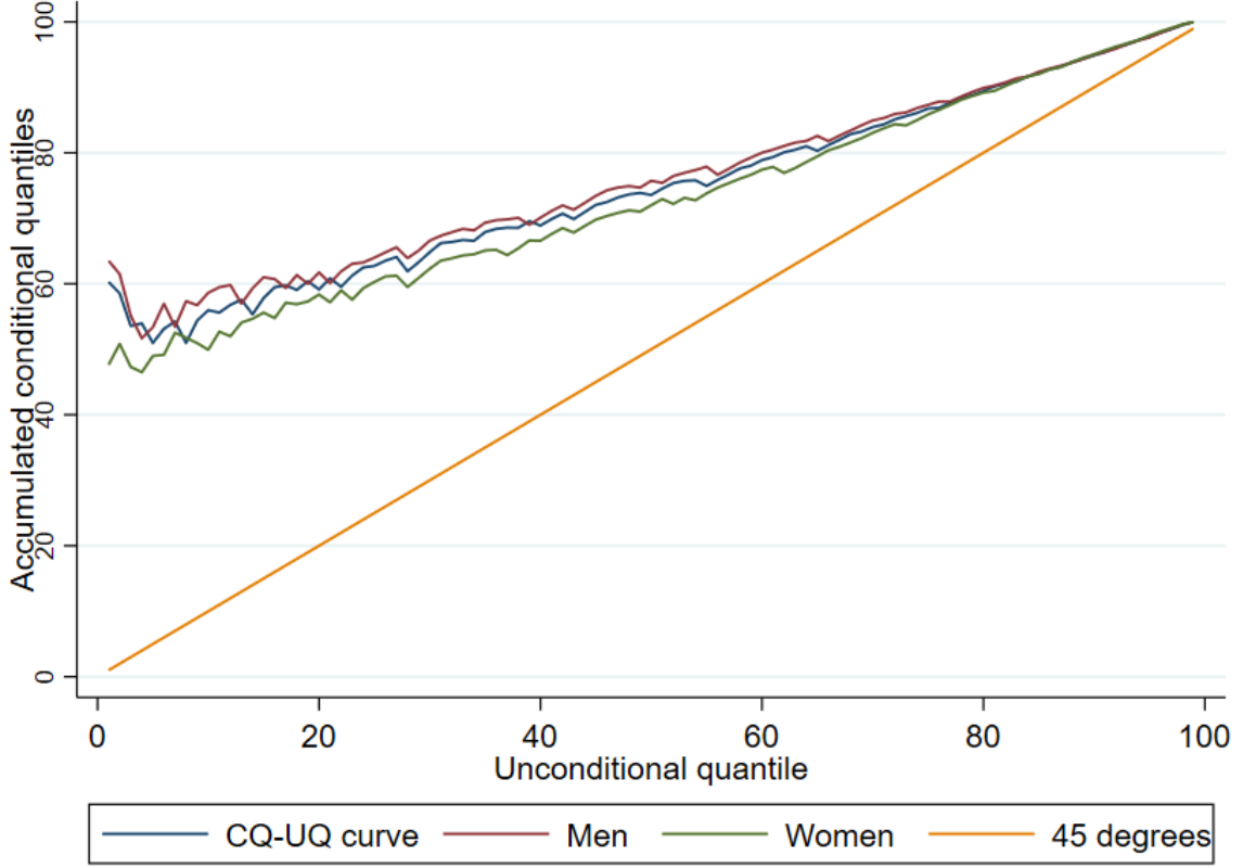
Figure 6: CQ-UQ, Gender Gap
